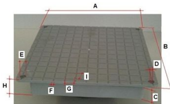
COVER DIMENSIONS
